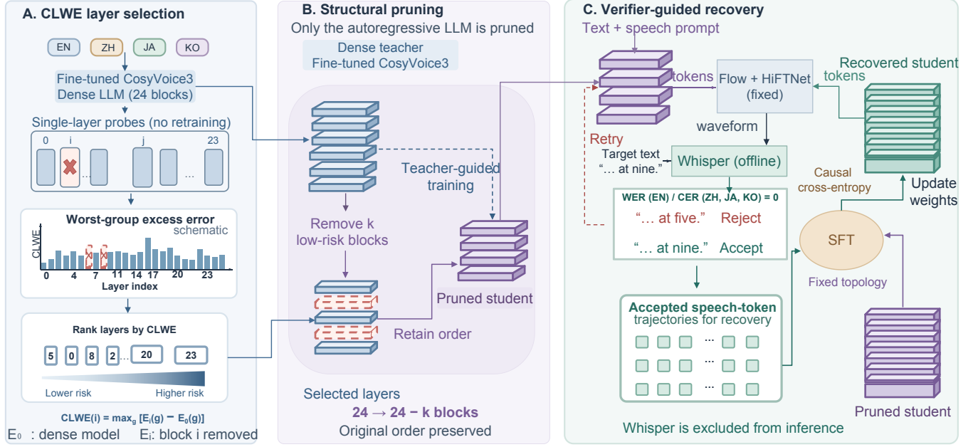
Fig. 1. Overview of CLWE-Prune. (A) Single-layer removal estimates cross-lingual worst-group excess risk. (B) We remove the lowest-scoring blocks and continue training the remaining model to obtain the Base checkpoint, while keeping the acoustic decoder fixed. (C) The pruned student is recovered on ASR-screened speech-token trajectories, keeping the pruning topology fixed.
